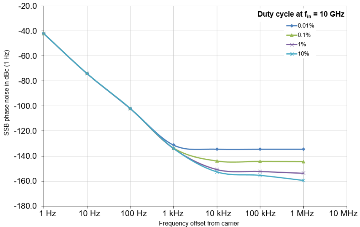
Typical phase noise sensitivity with R&S®FSWP-B60 or R&S®FSWP-B61 option at f_{in} = 10 GHz (start offset = 1 Hz, correlation factor = 1, signal level = 10 dBm, gating = on)
